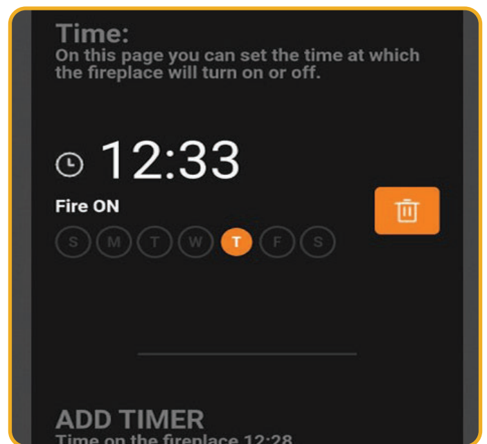
Fig. 2.4 | Timer Overview
