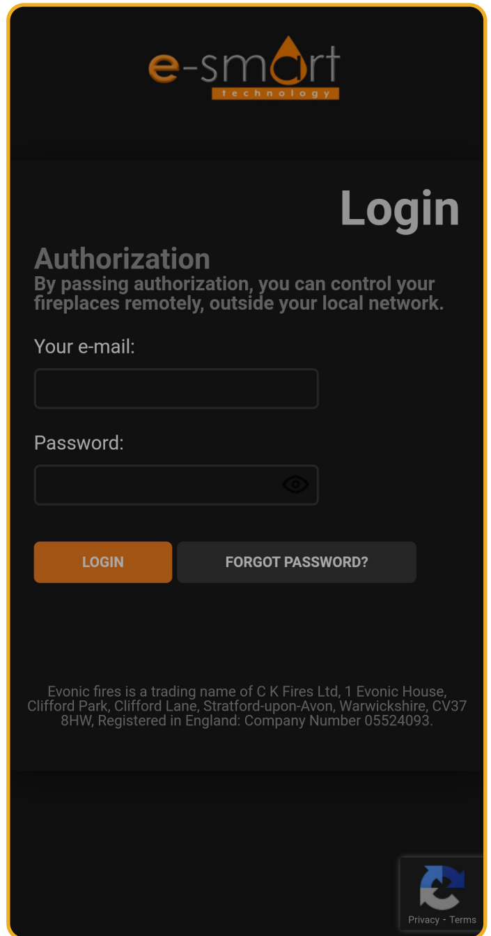
Fig. 2.5 | Login Screen
